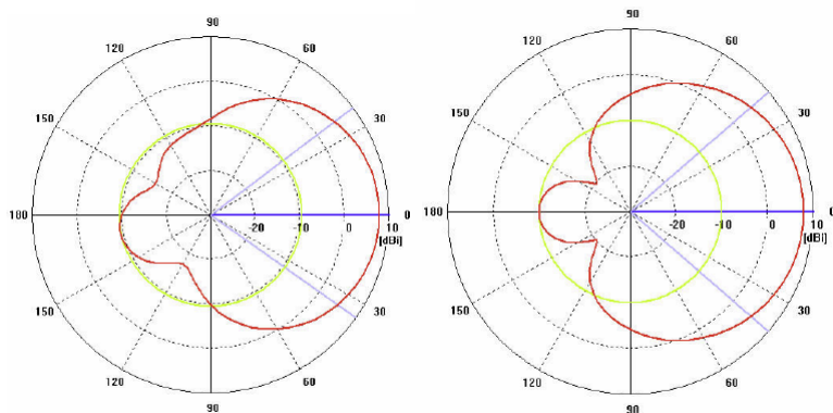
Vertical Radiation Pattern
