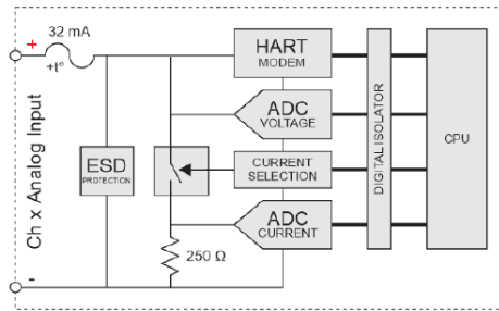
Analog Input Equivalent Circuit
